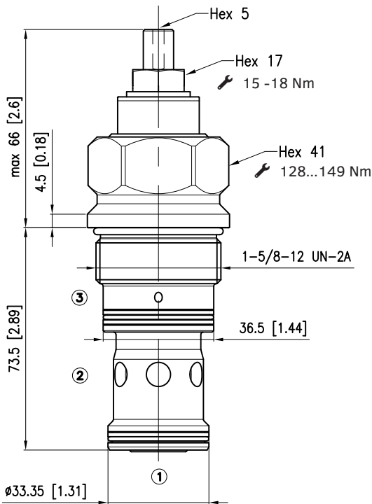
dimensions in mm [inch]
